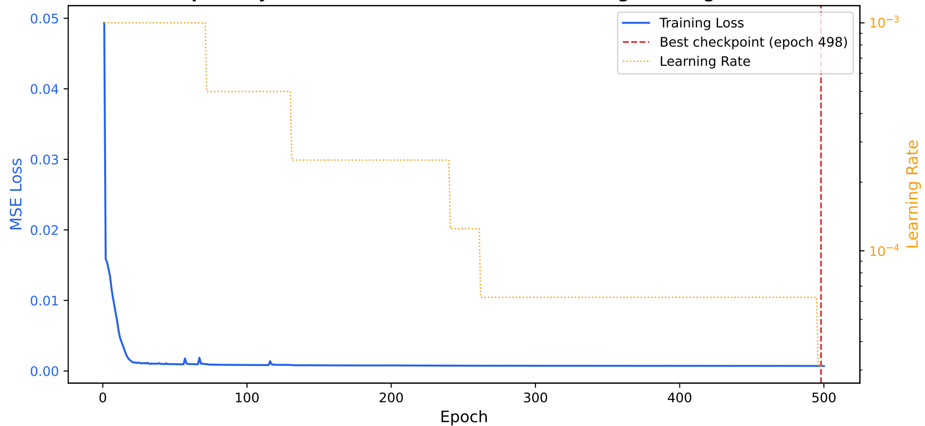
Triple-Projection Fusion Autoencoder — Training Convergence
